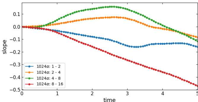
Figure: Plot of the slope of \max_{t \in [0, T^*]} \|\nabla u_{\alpha}\|_{L^2}^2 vs time.
