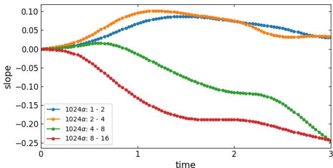
Figure: Plot of the slope of \max_{t \in [0, T^*]} \|\nabla \mathbf{u}_{\alpha}\|_{L^2}^2 vs time.
