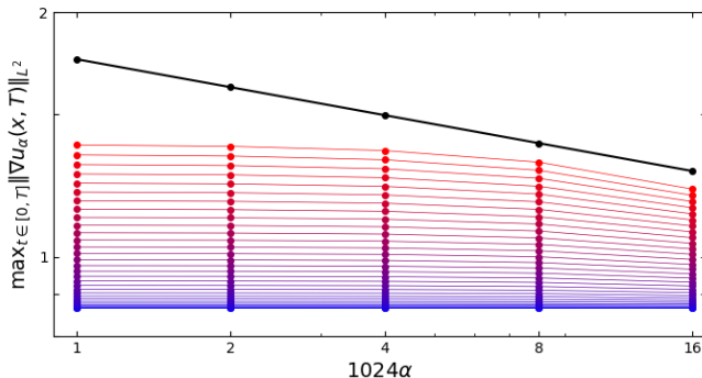
Figure: Log-log plot of \max_{t \in [0, T^*]} \|\nabla \mathbf{u}_{\alpha}\|_{L^2}^2 vs \alpha at T = 0 (blue) to T = 5.0 (red). C\alpha^P (black)
